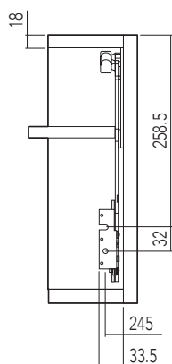
INT. FORATURA PER ANTA IN LEGNO INNER PART OF THE HOLE FOR WOODEN DOOR
