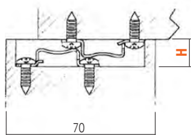
Scanalatura chiusa / closed pocket
