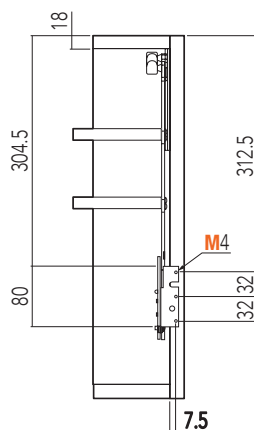
INT. FORATURA PER ANTA ALLUMINIO TELAI 20x20 INNER PART OF THE HOLE FOR ALUMINIUM DOOR 20x20
