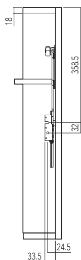
INT. FORATURA PER ANTA IN LEGNO INNER PART OF THE HOLE FOR WOODEN DOOR
