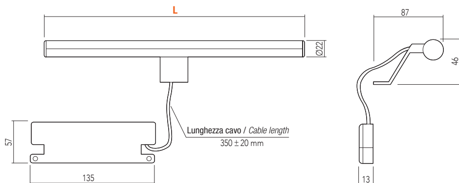
Supporto / support S2
