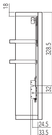
INT. FORATURA PER ANTA IN LEGNO INNER PART OF THE HOLE FOR WOODEN DOOR
