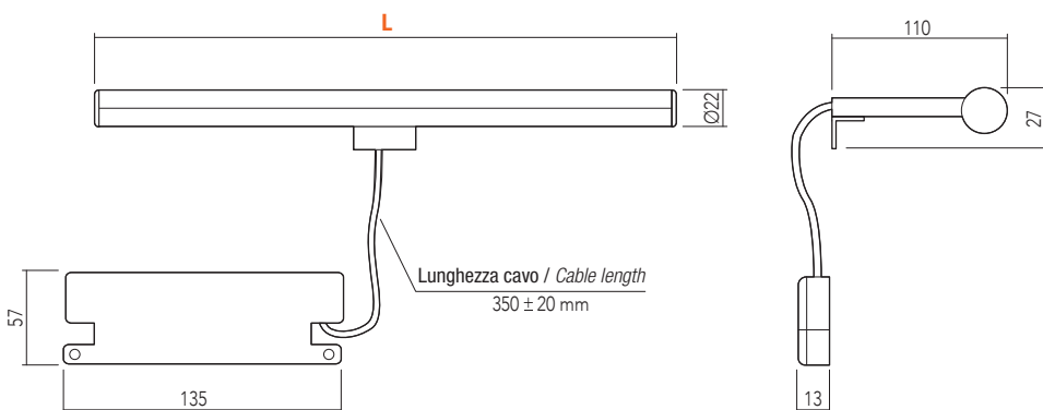
Supporto / support S3
