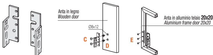
INT. FORATURA PER ANTA IN LEGNO INNER PART OF THE HOLE FOR WOODEN DOOR
