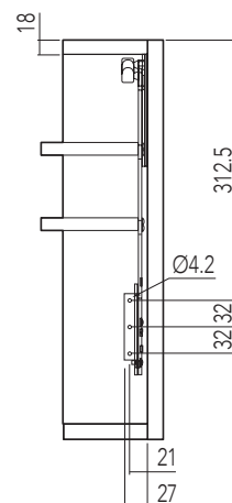
INT. FORATURA PER ANTA ALLUMINIO TELAI 45x20 INNER PART OF THE HOLE FOR ALUMINIUM DOOR 45x20
