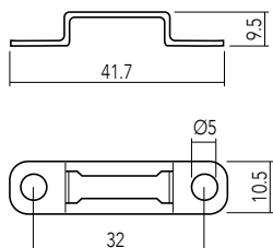
A clip passante / pass-thru
