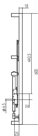
INT. FORATURA PER ANTA IN LEGNO INNER PART OF THE HOLE FOR WOODEN DOOR
