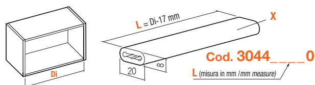
INT. FORATURA PER ANTA IN LEGNO INNER PART OF THE HOLE FOR WOODEN DOOR
