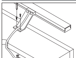
Supporto / support S2
