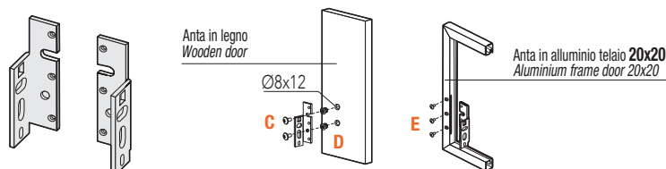
INT. FORATURA PER ANTA ALLUMINIO TELAI 20x20 INNER PART OF THE HOLE FOR ALUMINIUM DOOR 20x20
