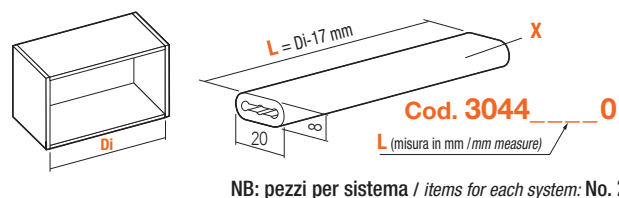
INT. FORATURA PER ANTA IN LEGNO INNER PART OF THE HOLE FOR WOODEN DOOR
